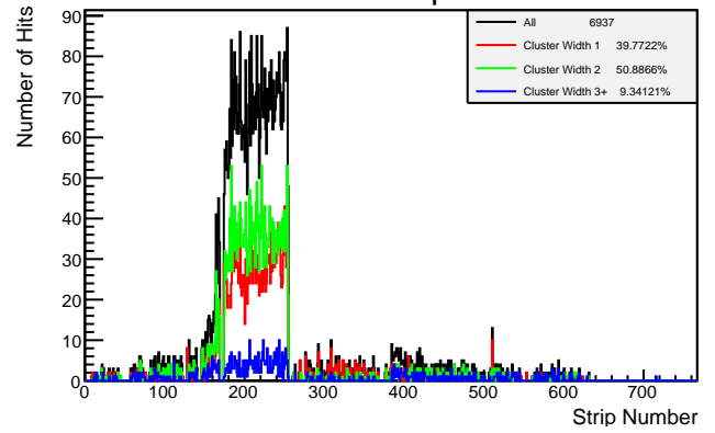
Cluster Noise
